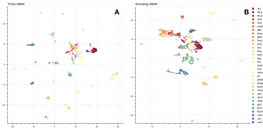
Fig. 3: UMAP projections of the RNA-Seq TCGA data (Figure 3A) and UFDN latent space encodings of said data (Figure 3B). The full 20,501 dimensional representation of gene expression levels have more cancer specific clusters, while the 100 dimensional latent space encodings have uncoupled from domain information, to some extent.
