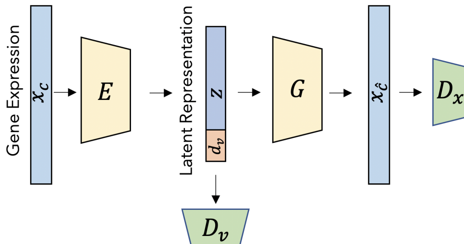
Fig. 2: The neural network architecture of UFDN-TCGA.
