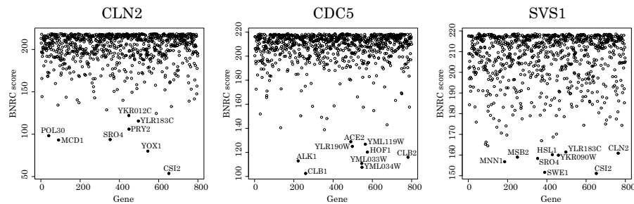
Figure 3: BNRC scores for CLN2, CDC5 and SVS1.
